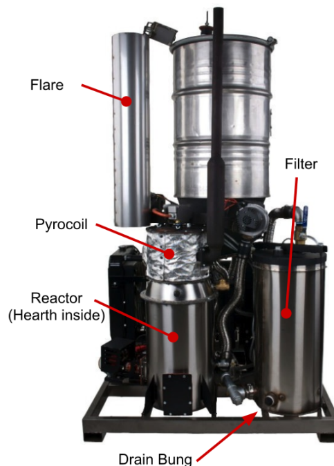
Reactor side of the Power Pallet
