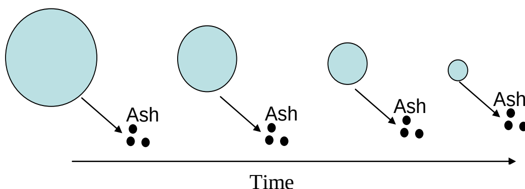
Figure 30. Particle Time History in Circulating Fluidized Bed Riser.
