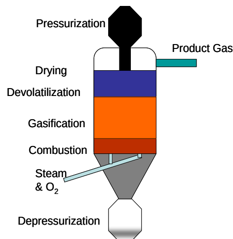
Figure 19. Typical Configuration for Dry and Slugging Moving Bed.
