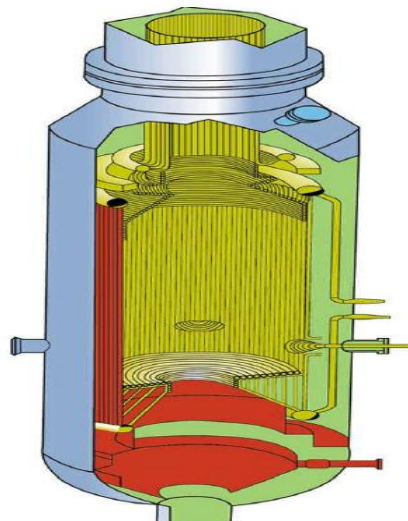
Figure 8. Shell Gasifier [1].
