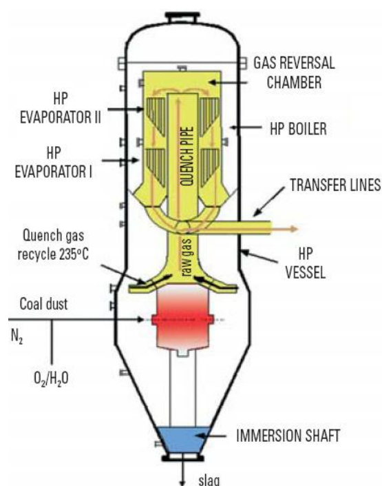
Figure 17. PRENFLO™ [1].
