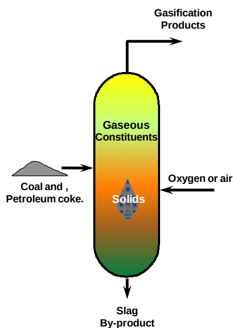
Figure 25. Typical Entrained Flow Gasifier [1].
