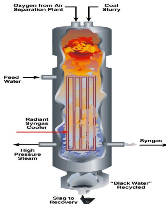
Figure 6. GE Energy Gasifier [1].
