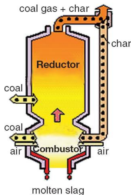
Figure 14. MHI Gasifier [1].
