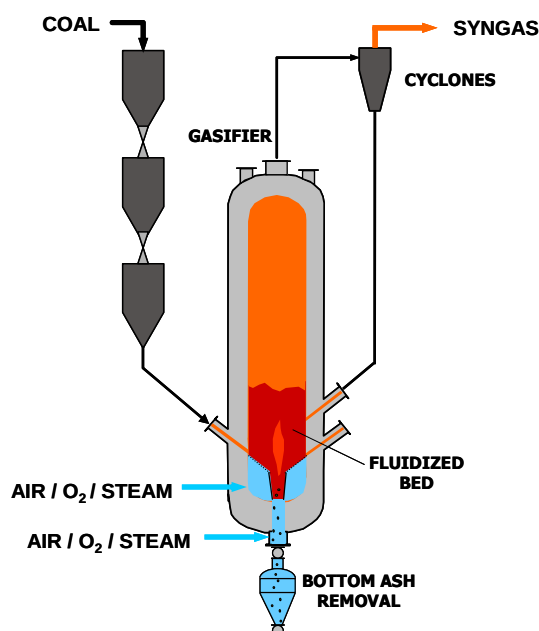
Figure 15. U-Gas Process [1].
