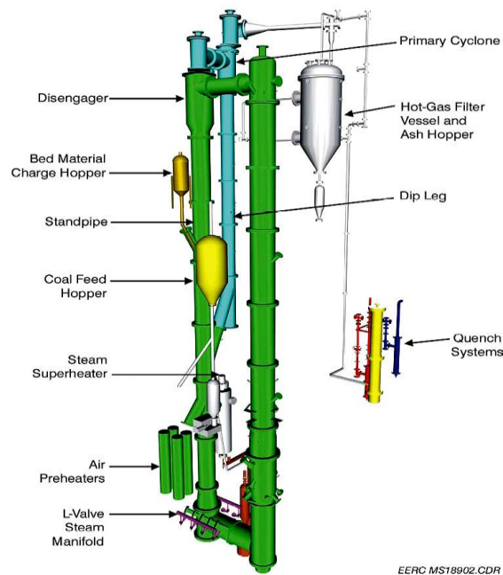
Figure 10. KBR Transport Gasifier [1].
