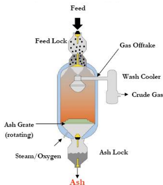
Figure 13. Lurgi Mark IV Gasifier [1].
