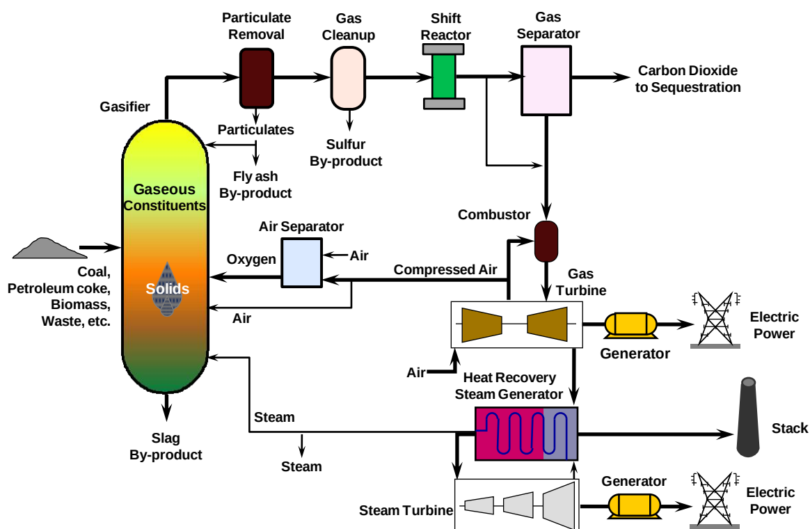
Figure 4. IGCC with carbon capture [1].
