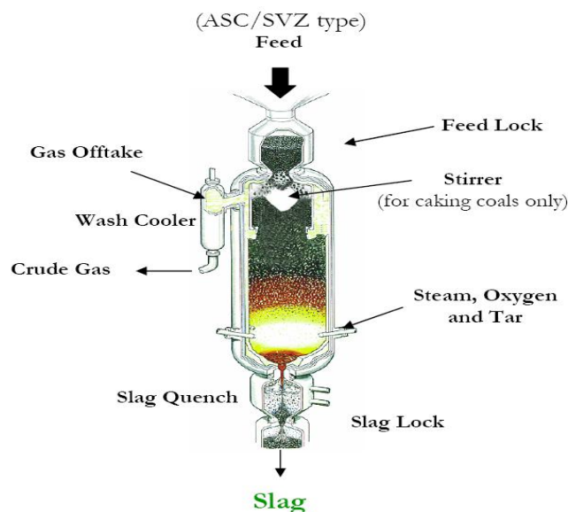
Figure 11. British Gas Lurgi Gasifier [1].
