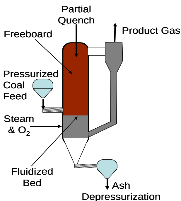
Figure 22. Fluidized Bed Gasifier Concept.
