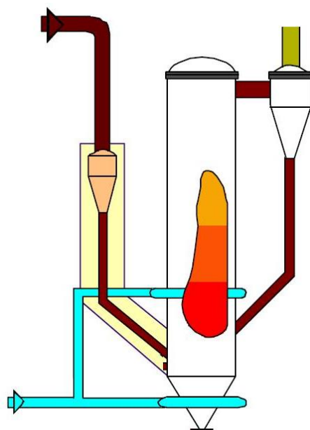
Figure 16. High Temperature Winkler Gasifier [1].
