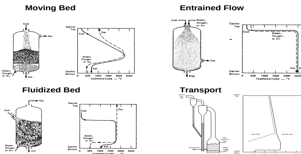
Figure 18. Gasifier Configurations [1].
