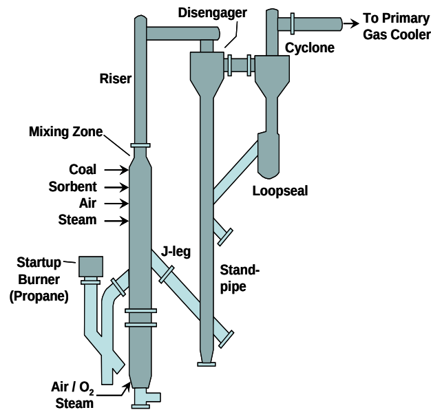
Figure 28. KBR Transport Gasifier.
