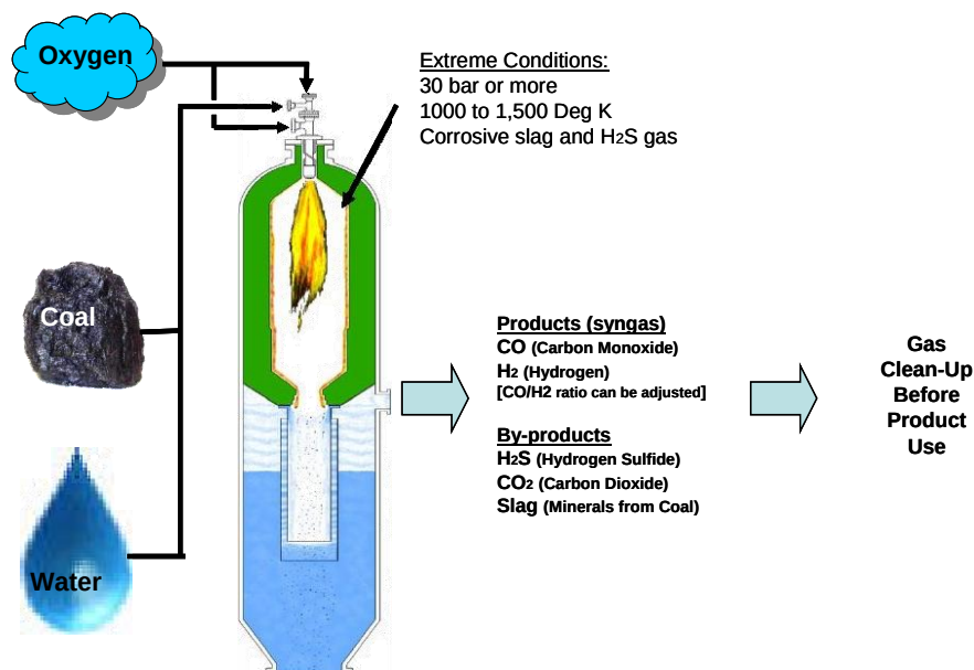
Figure 1. Gasification process basics.
