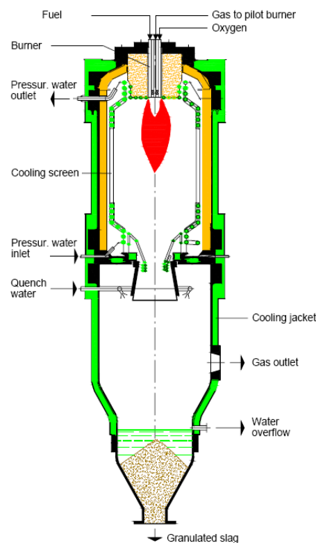
Figure 9. Siemens Gasifier [1].
