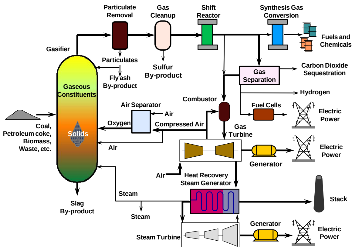
Figure 5. Poly-generation plant [1].
