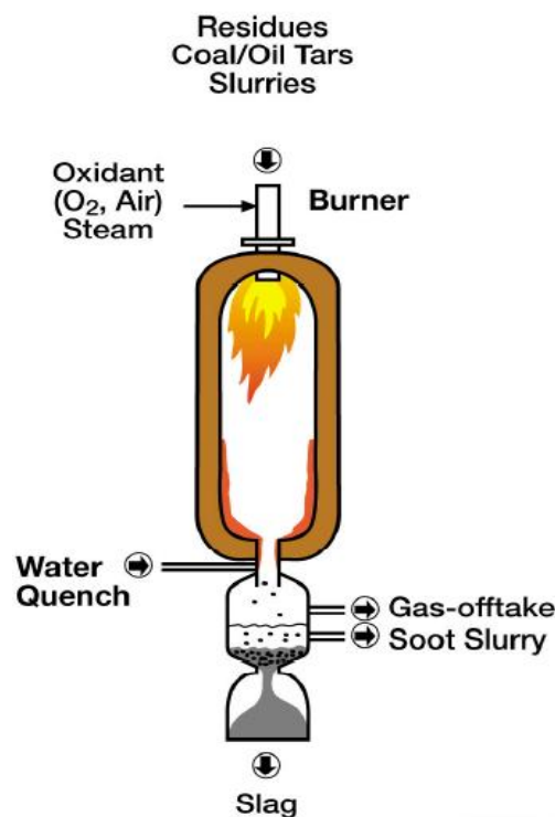
Figure 12. Lurgi Multi Purpose Gasifier [1].
