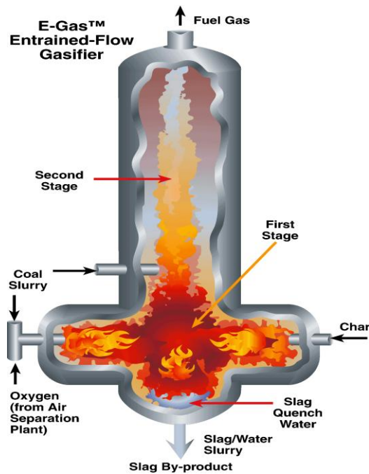
Figure 7. Conoco Philips E-Gas [1].
