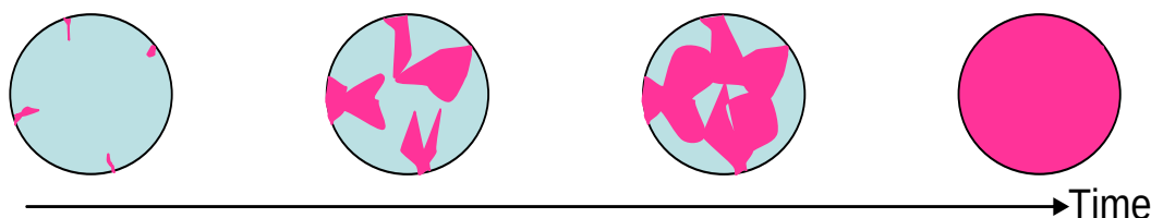
Figure 27. Bulk Diffusion Controlled Conversion in Entrained Flow Gasifiers.
