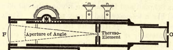
FIG. 18. — Féry's Thermo-electric Telescope.
