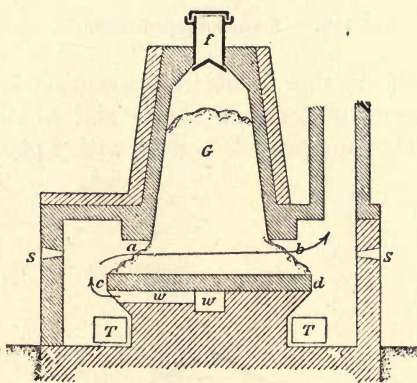
FIG. 109. — Generator of Tholander.
