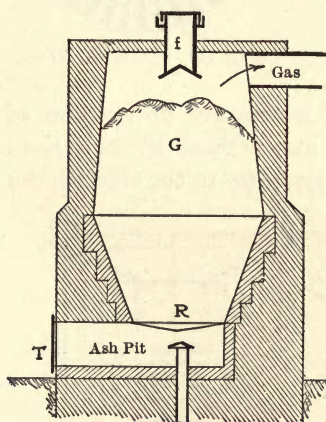
FIG. 108. — Odelstjerna's Generator for Peat, Wood and Shavings.
