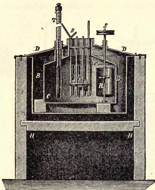
FIG. 7. — Weinhold's Pyrometer.
