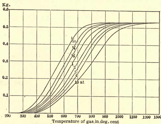
FIG. 92. — Gasification of Carbon by Steam.
