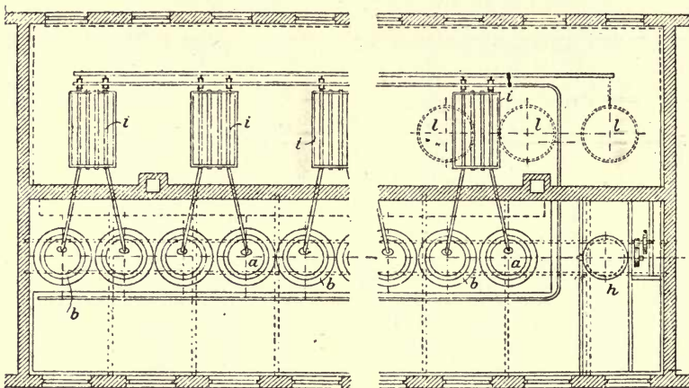
FIG. 55. — Plan of a Modern Charring Plant with Vertical Retorts.
