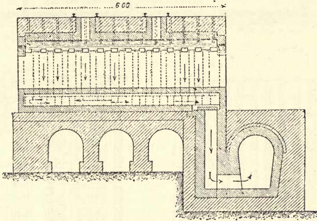
FIG. 73. — Coke Oven, François (longitudinal section).
