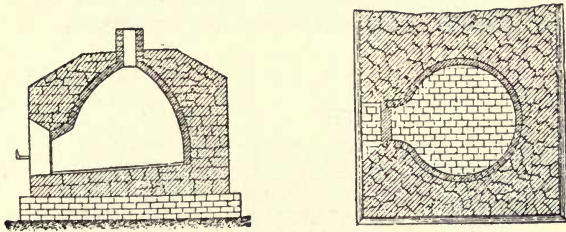
FIGS. 62 and 63. — Riesa Oven.
