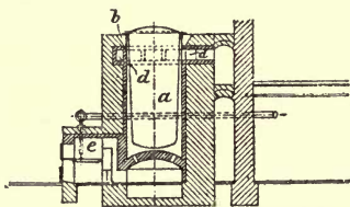
FIG. 56. — Modern Charring Plant with Vertical Retorts.
