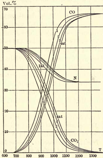
FIG. 84. — Ideal Composition of Generator Gas from 50 per cent Oxygen.
