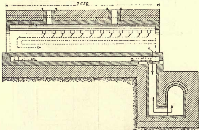
FIG. 67. — Section of Francois-Rexroth Coke Oven.
