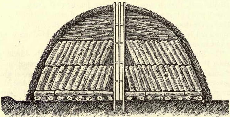
FIG. 34. — Italian Pile.
