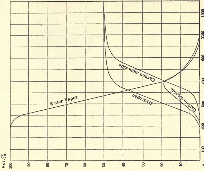
Fig. 88. — Ideal Composition of Water Gas at 3 Steam Pressure of 4 Atmospheres.
