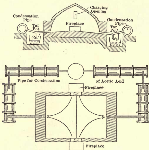
Figs. 40 and 41. — Schwartz Oven.
