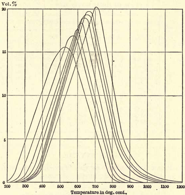
FIG. 91. — \text{CO}_2 in Water Gas.
