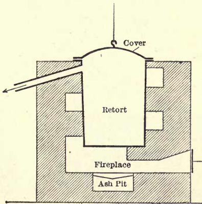
FIG. 43. — Section through French Oven heated from the Outside.
