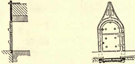
FIGS. 70 and 71. — Coke Oven, System Smet (details of doors).
