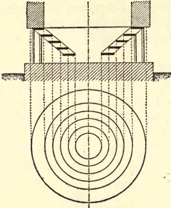
FIG. 110. — Funnel-Shaped Grate.
