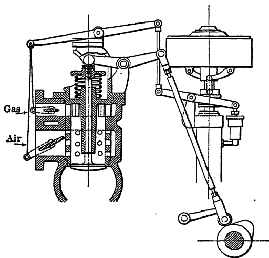
FIG. 107.—Constant-Quantity Regulation
