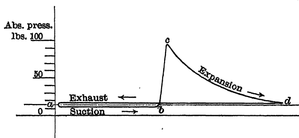
FIG. 8.—Indicator Card from Lenoir Engine.
