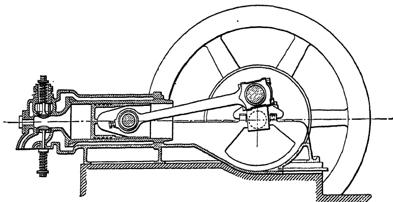
FIG. 9.—Sectional Elevation. Otto Engine.
