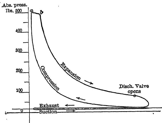
FIG. 13.—Indicator Card from Diesel Engine.
