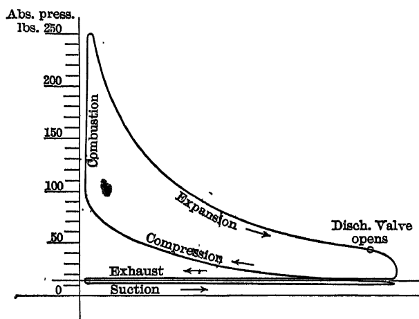
FIG. 10.—Indicator Card from Otto Engine.
