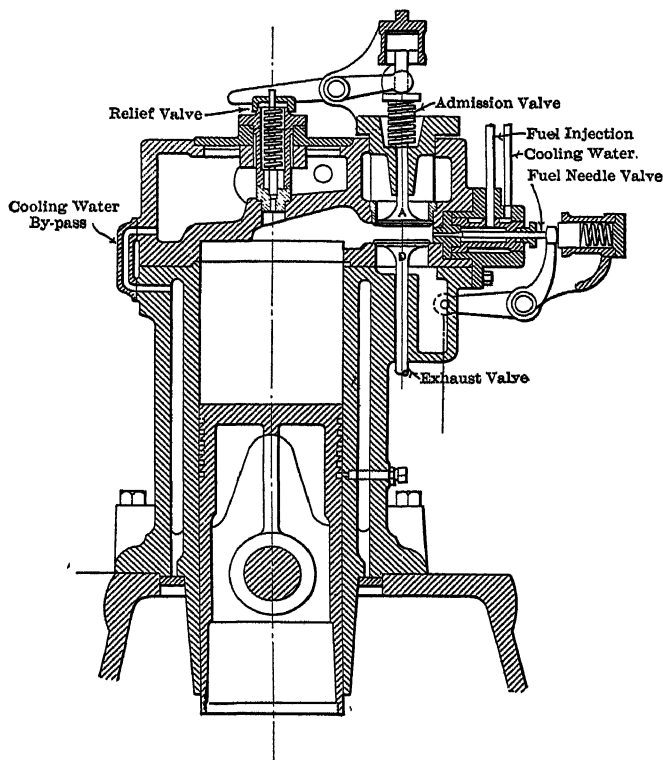
FIG. 12.—Section through Diesel Cylinder.
