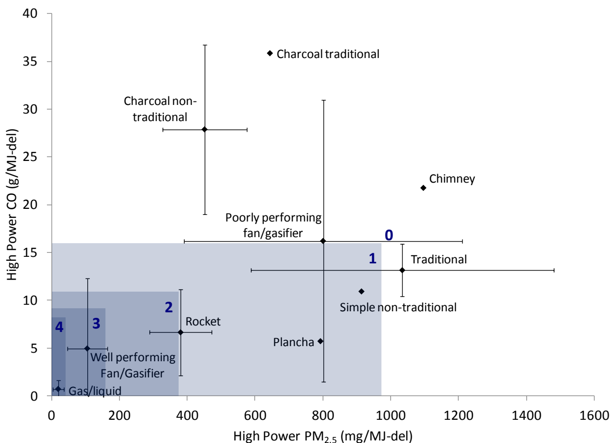
Figure 5. High power emissions performance for key stove/fuel classes across the IWA Tiers for the WBT. Error bars represent ± one standard deviation of the available tests sets. Stove/fuel classes with no error bars consist of two or less data points. Tiers are indicated by blue numbers.
